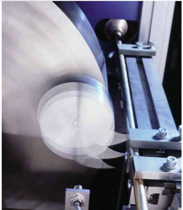
Cyclo-cutter
